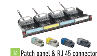
16 Patch panel & RJ 45 connectors
